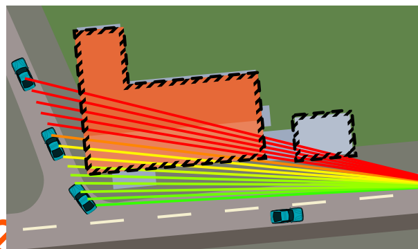
Fig. 1: Deterioration of received signal strength (RSS) as a transmission is blocked by first one, then two buildings. Input parameters of the presented model are the buildings' geometries and the positions of both the sending and the receiving node.
